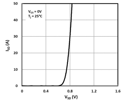
Fig.5 Source-to-drain diode forward characteristics
