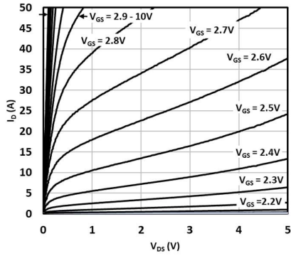
Fig. 1 Output characteristics
