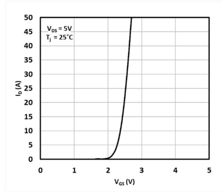
Fig. 2 Transfer characteristics
